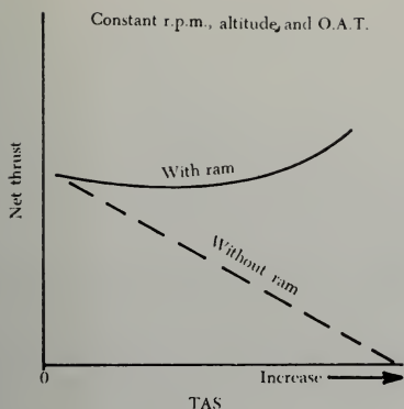
FIGURE 1-76. Effect of airspeed on net thrust.
